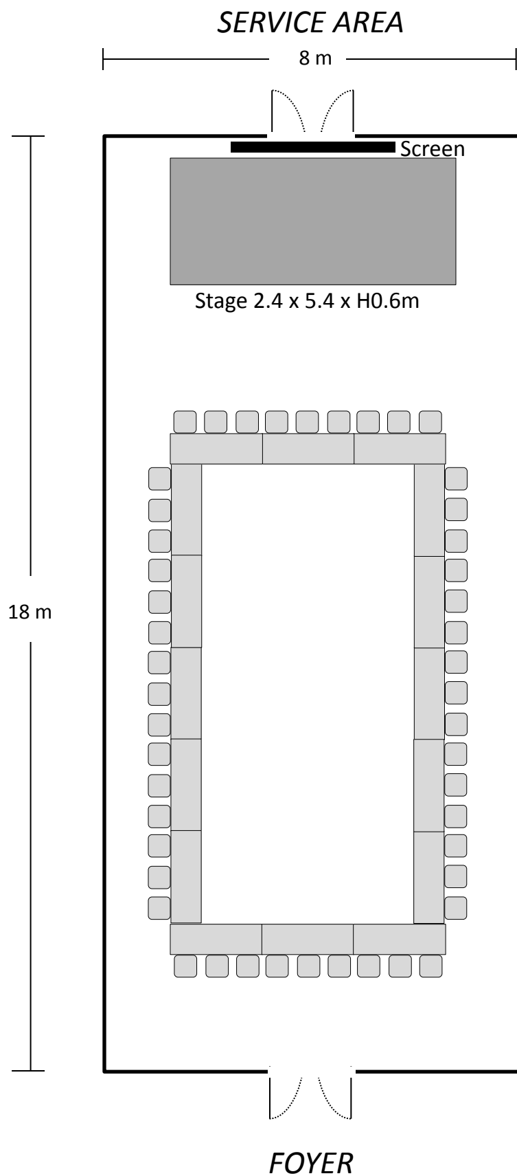
LEELAWADEE 1/2/3/4/5 HOLLOW SQUARE SETTING – 48pax 144sqm – 8 x 18m
